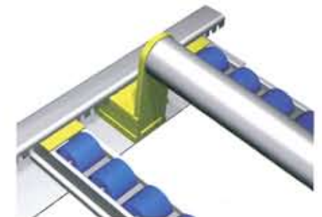
A full length divider keeps all goods in line and avoids carton damage.
