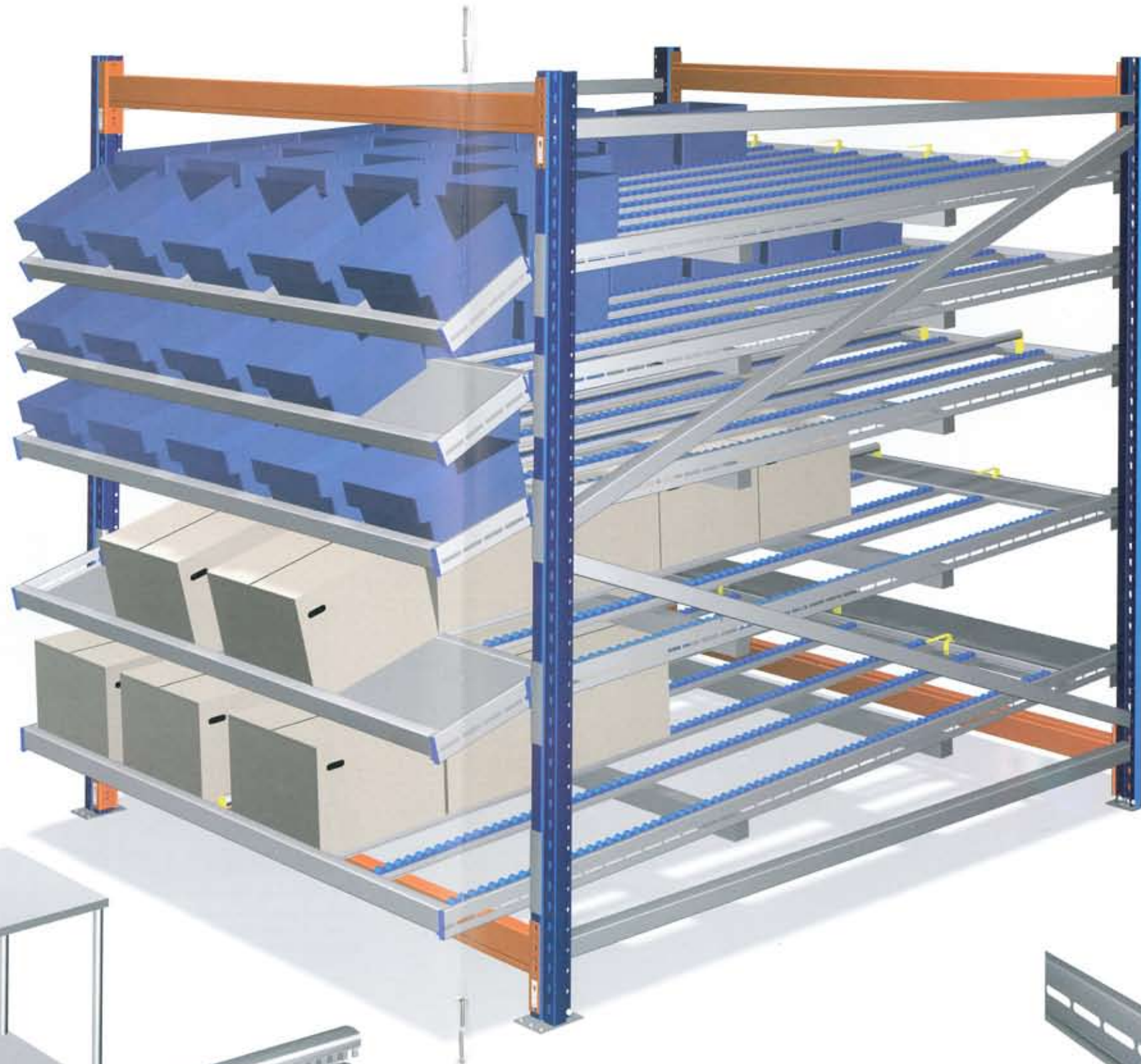
Entrance guides make loading a simple matter.
